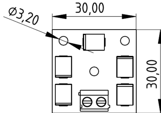
Figure 2: Dimensions of the module (all dimensions in mm).
